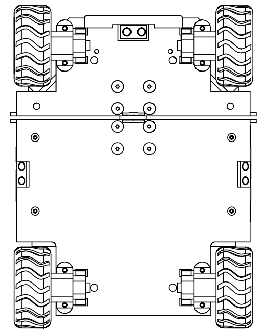
VIEW BOTTOM
