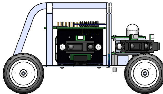
VIEW LEFT
