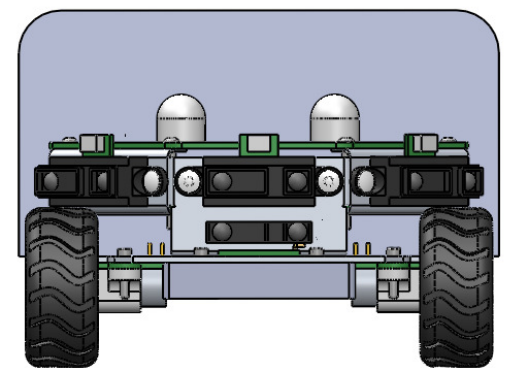
VIEW FRONT
